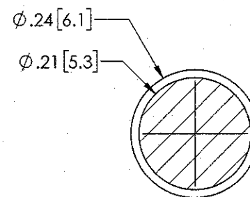
SECTION B-B SCALE 4:1
